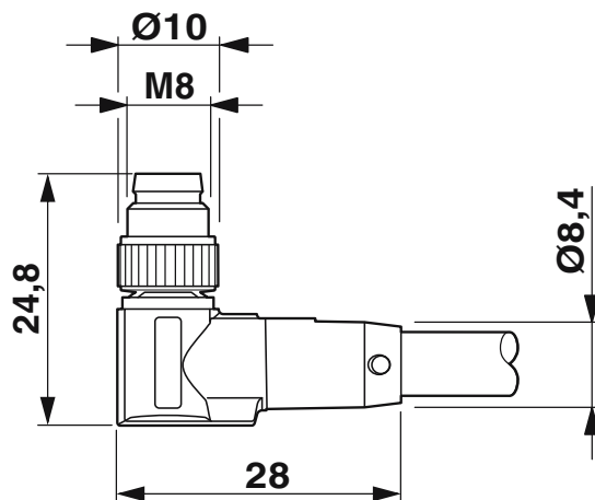
Dimensional drawing
